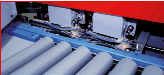
Polieraggregat buffing unit
