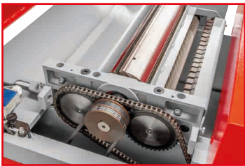
massiver Lagerblock solidly bedded cutter block
