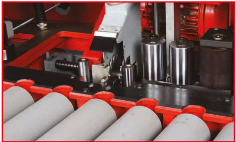
Sägeaggregat sawing device
