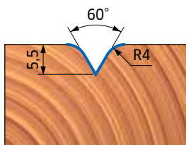
PROFILE / PROFILO 1
