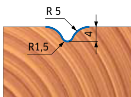
PROFILE / PROFILO 5
