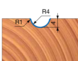
PROFILE / PROFILO 2
