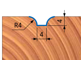
PROFILE / PROFILO 6
